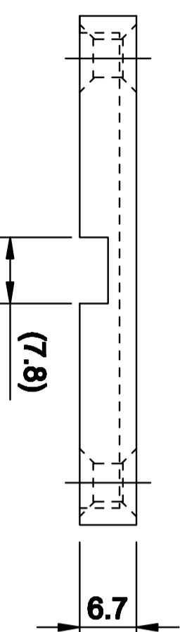
RETAINER
